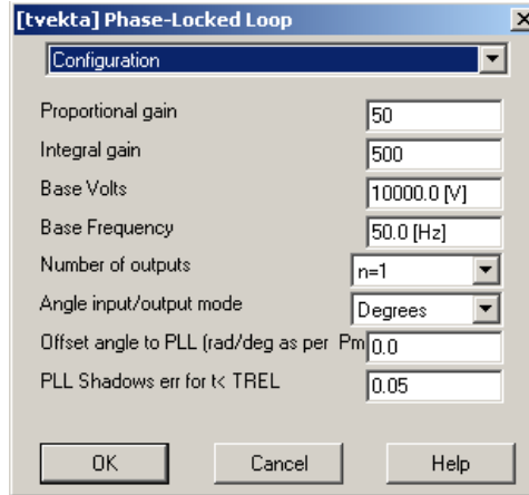
Figure 63: PLL characteristics
