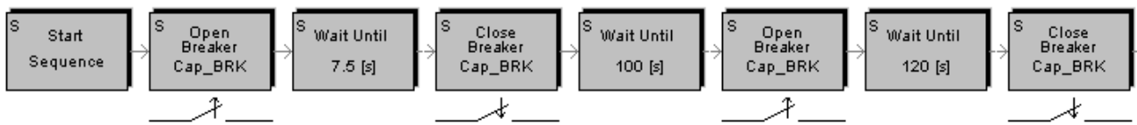
Figure 50: Add two breaker operations to limit current peak at 2nd capacitance charging
