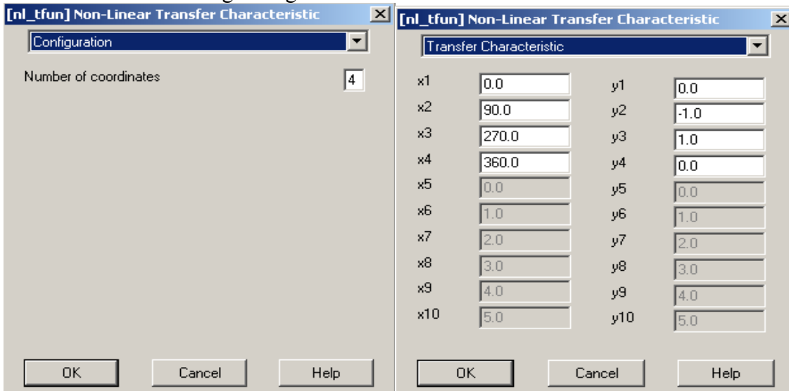
Figure 65: 2 nd Non linear transfer function characteristics
