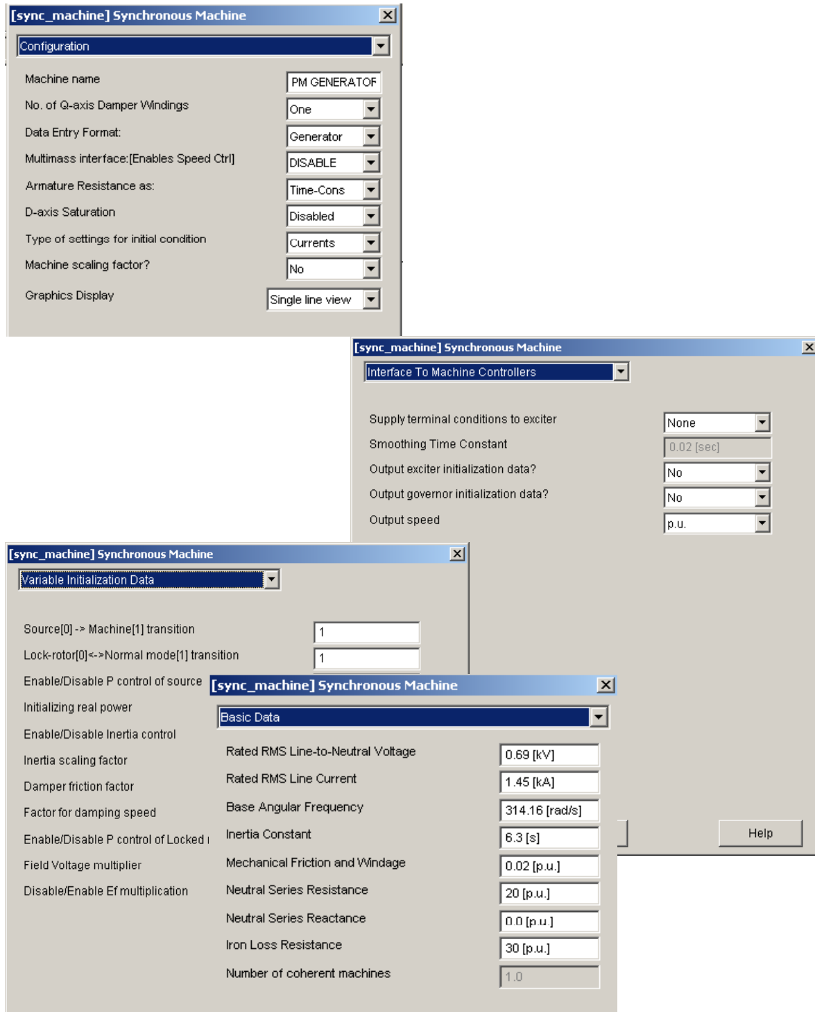
Figure 8: Synchronous machine characteristics
