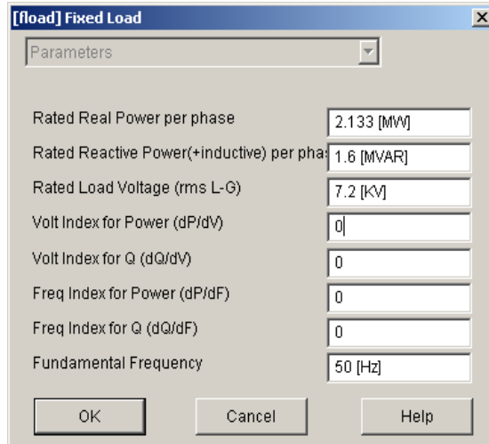
Figure 32: Node 1 load characteristics
