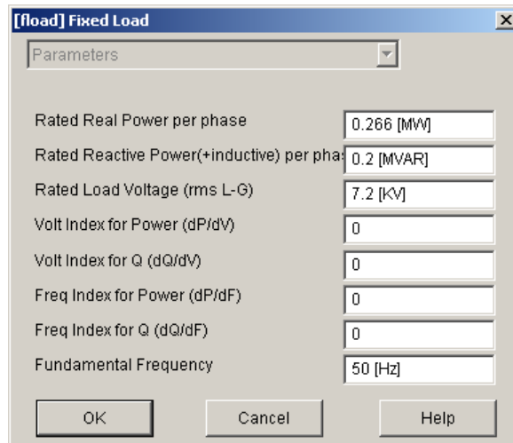
Figure 33: Node 2, 3 load characteristics
