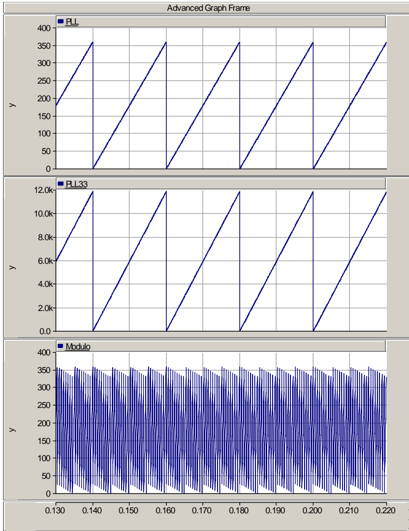
Figure 68: PLL output
