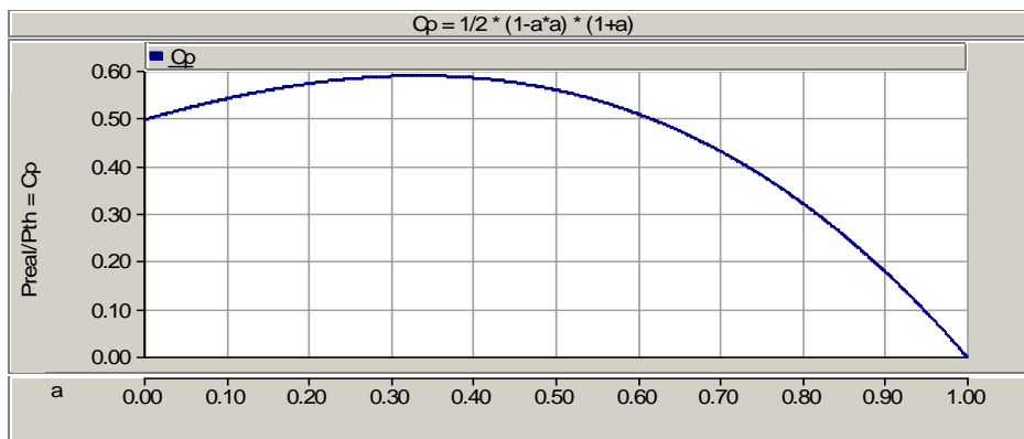
Figure 2 : Theoretical Cp(a)
