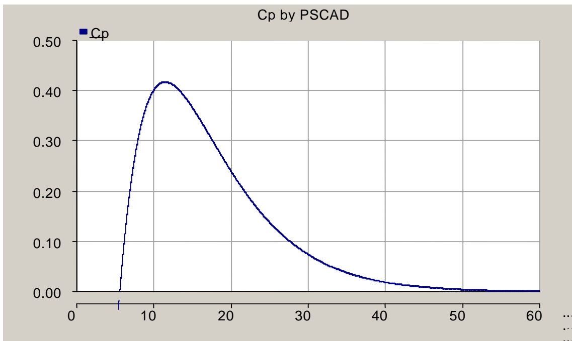
Figure 4: PSCAD C_p(\gamma)
