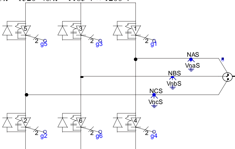
Figure 57: 6 pulse bridge GTO inverter
